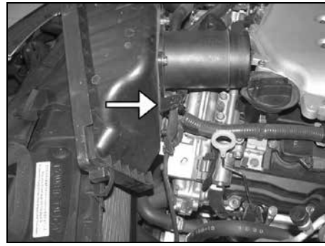
7. Unclip the air cleaner lid, then, loosen and remove the single bolt that secures the air cleaner lid to the fender. Rotate the air cleaner lid, then, unclip the mass air sensor electrical connection to remove the air cleaner lid as shown.
