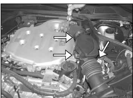
4. Loosen the hose clamps at the throttle body and at the mass air sensor, then, loosen and remove the bolt that secures the resonator to the intake manifold.
